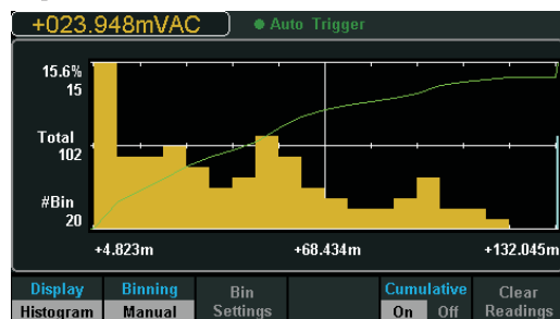
Histogram
