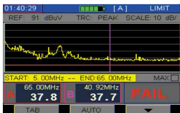
Return Path Spectrum (5-65)
