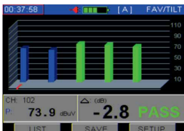
Tilt (Max 12 Freq.)
